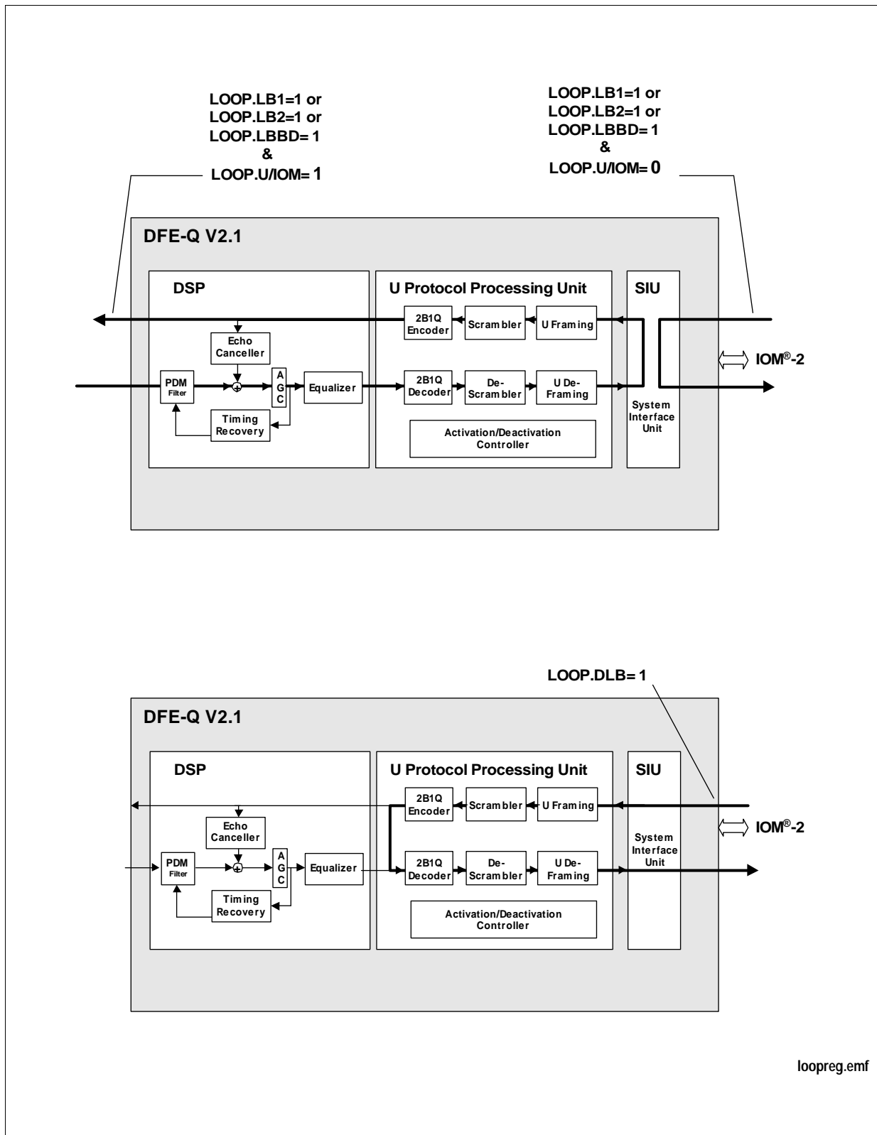
Figure 2 Loopbacks Featured by Register LOOP
